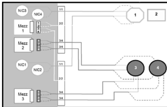
c3000 Full Height Server Blade
