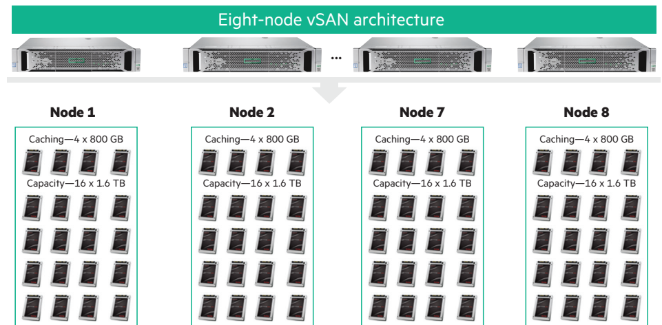
Figure 1. HPE All-Flash vSAN Solution
