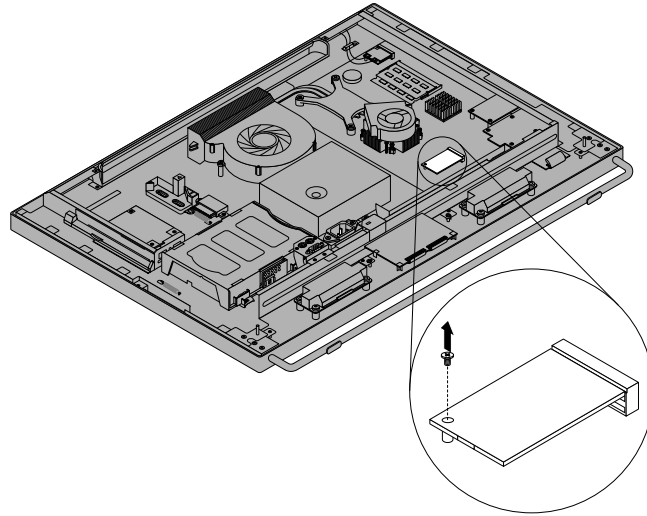
Figure 40. Removing the screw that secures the mSATA solid-state drive or mini PCI Express x1 card
