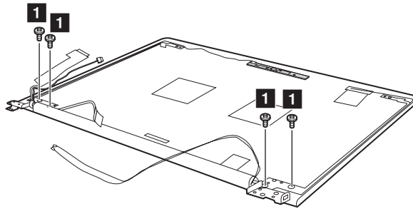
Figure 14. Removal steps of hinges
